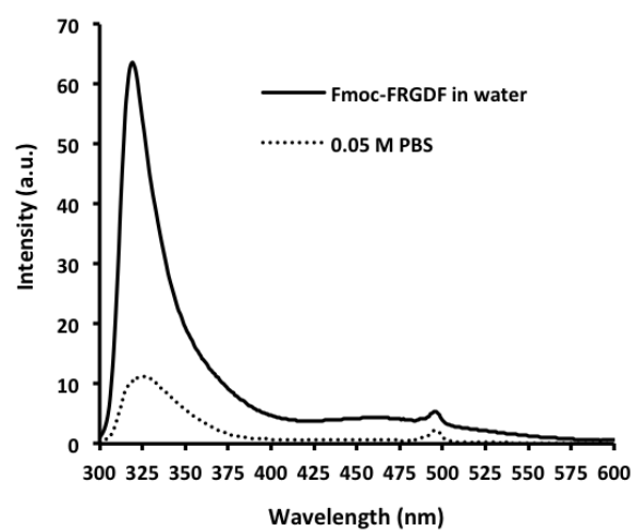
Supplementary Figure 1 Fluorescence spectrum of Fmoc-FRGDF hydrogel.
