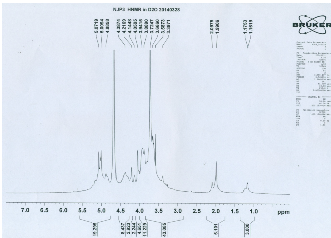
^1\text{H} NMR spectrum of HJP3
