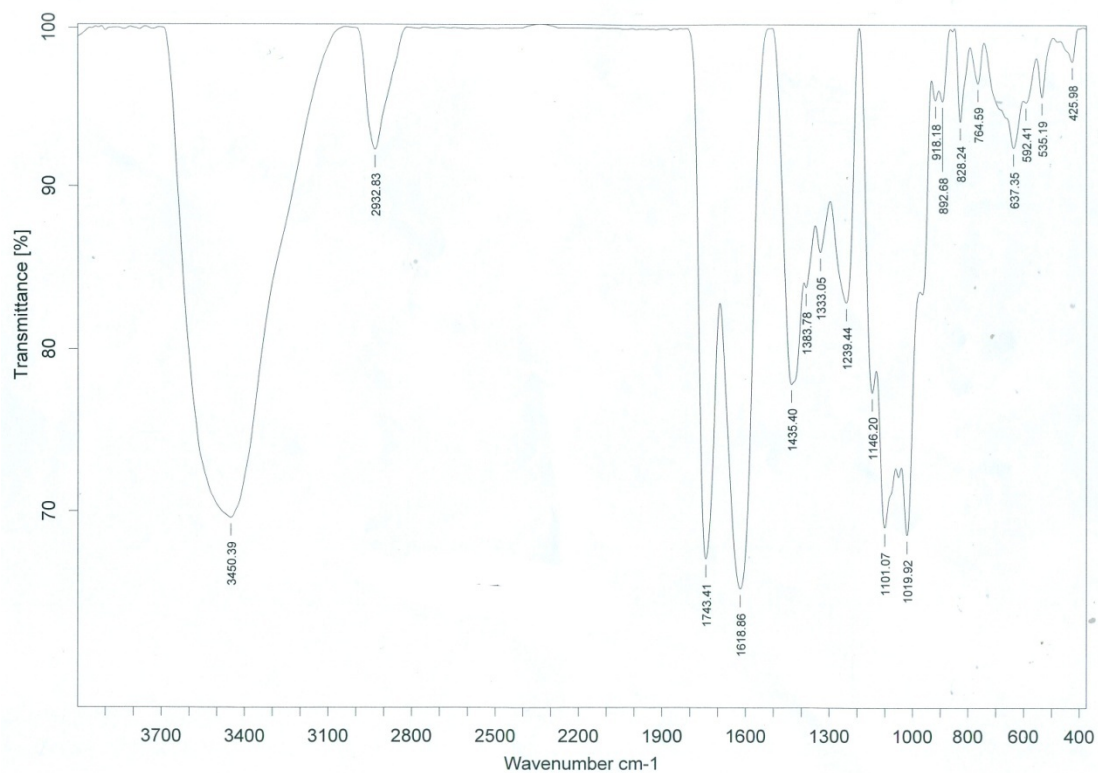
IR spectrum of HJP3
