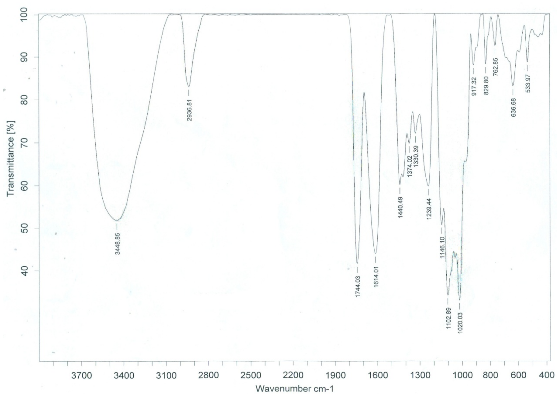
IR spectrum of HJP1
