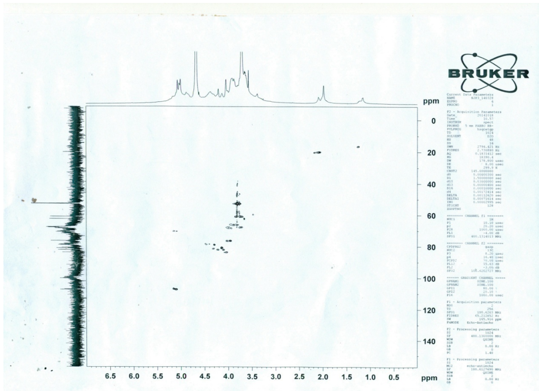
HMQC spectrum of HJP3
