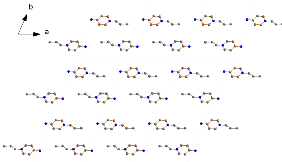
Figure S1 The stacking patterns of cations of 1 (hydrogen atoms are omitted for clarity).
