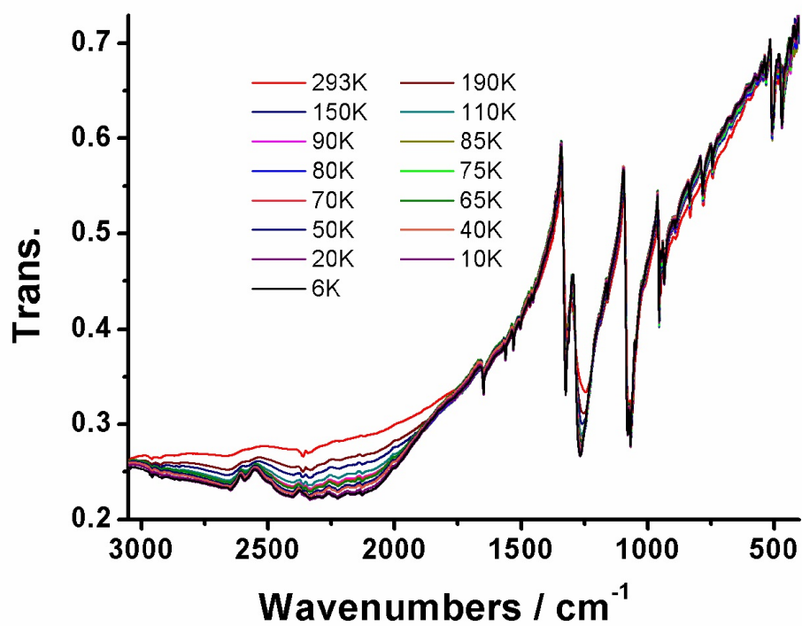
Figure S2 Temperature dependent IR spectra of 1 .
