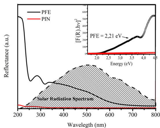
Figure S1. Diffuse reflectance spectra and the band gap calculation for PIN (red line) and PFE (black line). Kubelka-Munk function on the detail.
