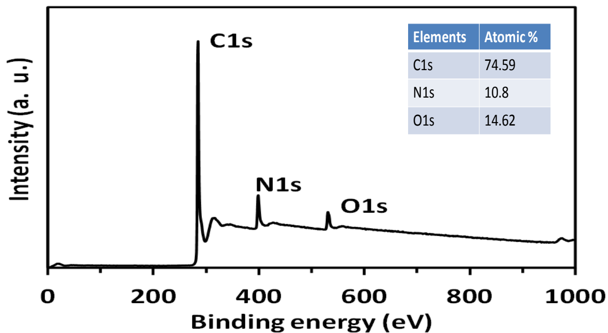
Figure S3 XPS survey spectra of N-GO coatings
