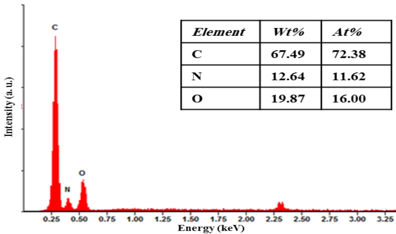
Figure S4 EDX analysis of N-GO coatings
