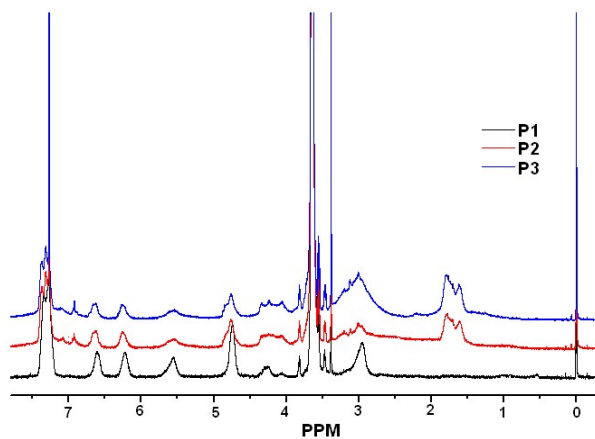
Figure S2. The 1 H NMR spectra of P1, P2, P3.
