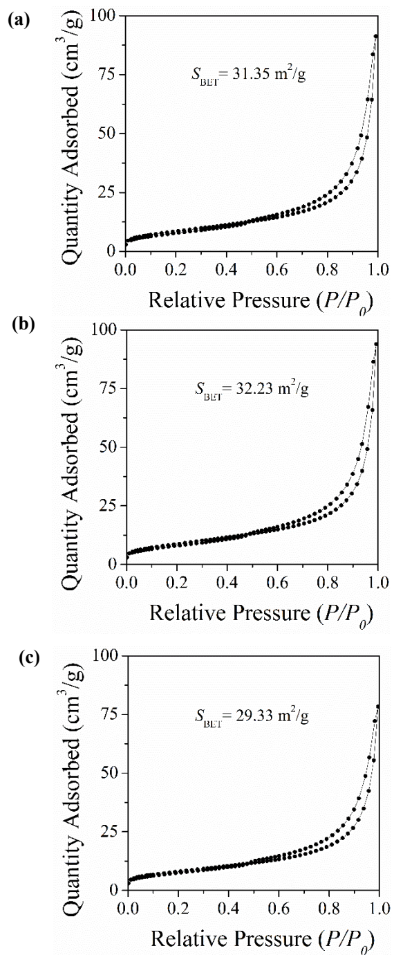
Figure S1 N 2 adsorption-desorption isotherm of C600-Mt (a), C700-Mt (b) and C800-Mt (c).
