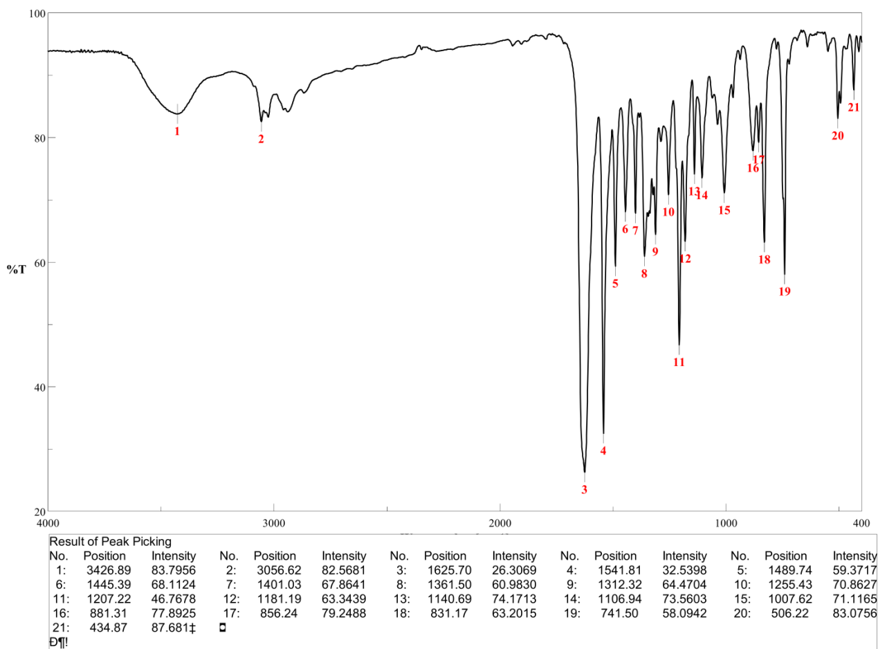
Fig. 1-S-1. IR spectrum of H 2 NAPPR (KBr pellet).
