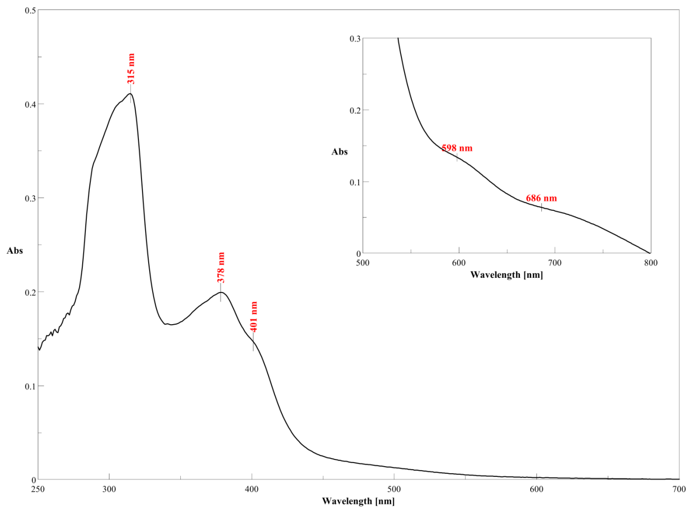
Fig. 2-S-2. UV-Vis spectrum of [\text{Cu}_2(\mu\text{-NAPPR})(\mu_{1,1}\text{-N}_3)_2]_n in DMF solution.
