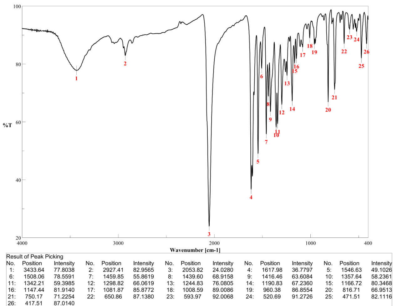
Fig. 1-S-2. IR spectrum of [\text{Cu}_2(\mu\text{-NAPPR})(\mu_{1,1}\text{-N}_3)_2]_n (KBr pellet).
