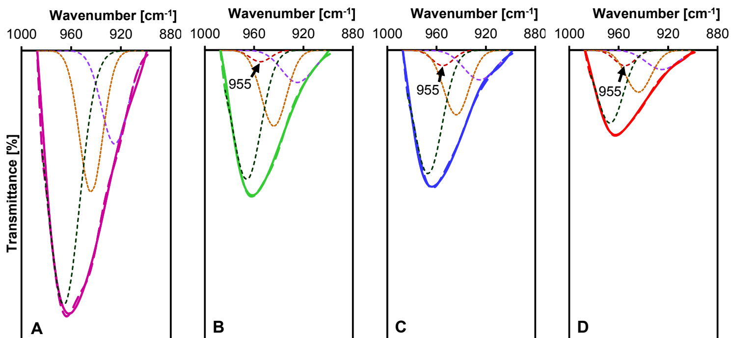
Figure S2. FT-IR spectra of (A) MSN, (B) 5wt% IS-FeOOH/MSN, (C) 10wt% IS-FeOOH/MSN and (D) 15wt% IS-FeOOH/MSN and Gaussian curve-fitting of band at 960 cm -1
