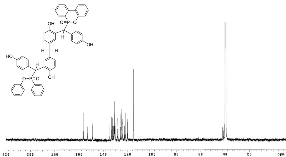
Figure S1. 13 C-NMR spectrum of (3).
