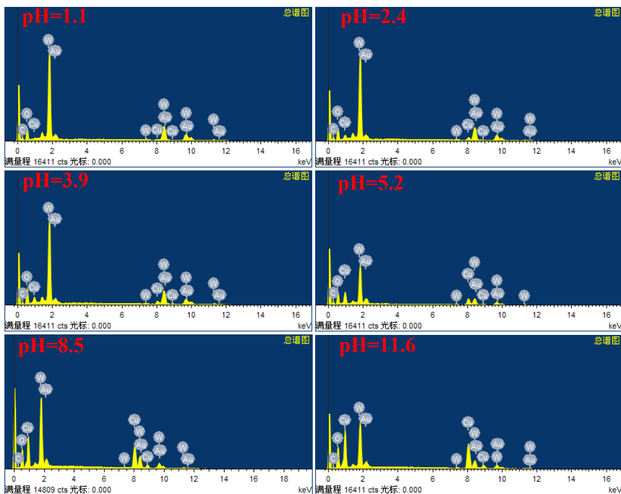
Fig. S1. EDS spectra of the samples prepared at different pHs.
