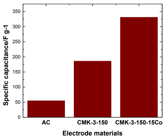
Fig. S1. Variation specific capacitance of AC, CMK-3-150 and CMK-3-15-15Co electrodes.
