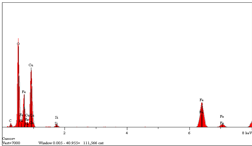
Fig. 1 The EDX spectrum of native \text{CuFe}_2\text{O}_4 catalyst
