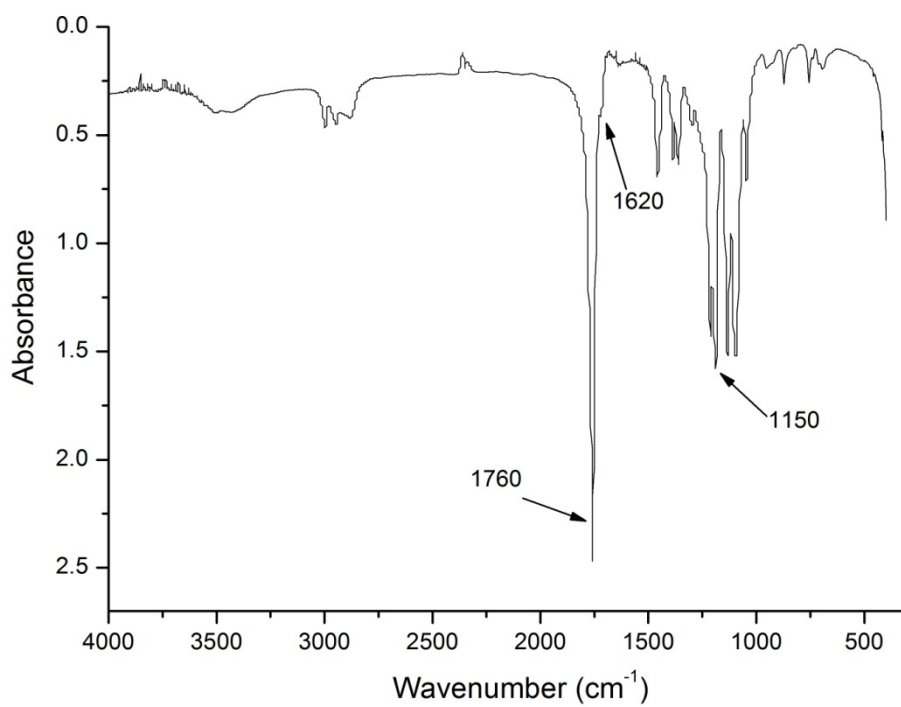
Fig. S1 FTIR spectrum of PLA-PEG methacrylate copolymer
