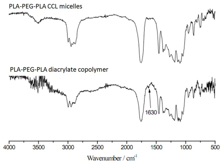
Fig. S3 FTIR spectrum of PLA-PEG-PLA CCL micelles and uncross-linked micelles
