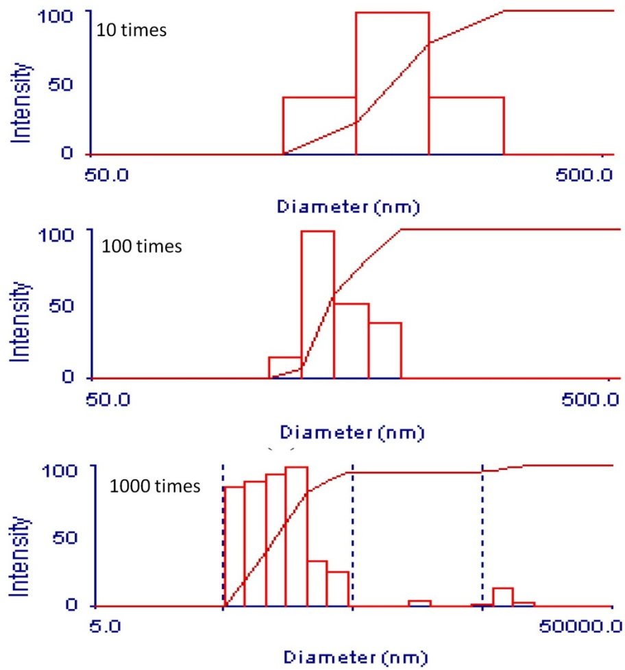
Fig. S6 Size distributions curves of PLA-PEG-PLA CCL micelles after diluting with different times
