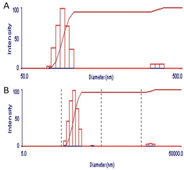
Fig. S4 Polydispersity of PLA-PLA uncross-linked micelles (A) and PLA-PEG SCL micelles
