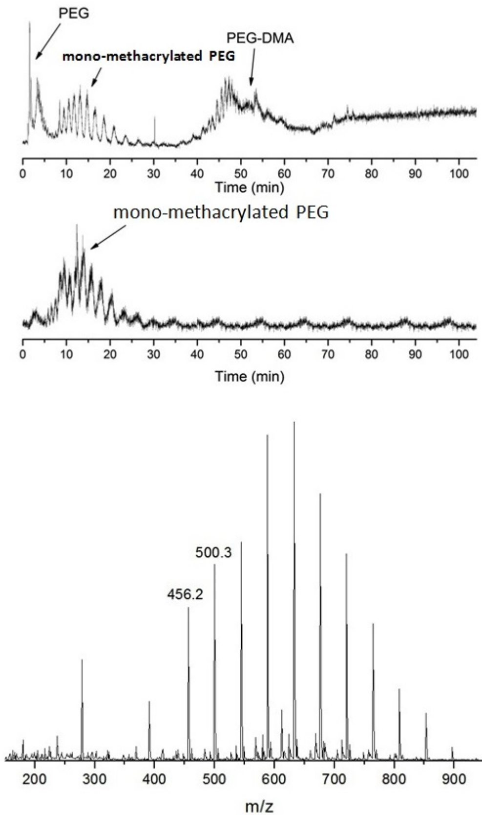
Fig. S2 (A) HPLC chromatograms of PEG-MIX and mono-methacrylate PEG, (B) Mass spectroscopy of PEG-MMA
