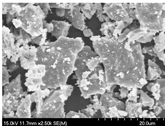
Figure S1 SEM image of the host \text{Mg}_2\text{Y}_2\text{Al}_2\text{Si}_2\text{O}_{12} .
