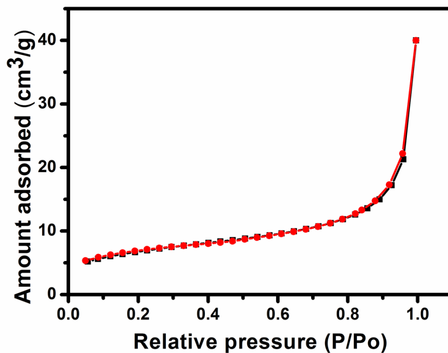
Fig. S1 The BET spectra of the precursor \text{Co}_2\text{CO}_3(\text{OH})_2 .
