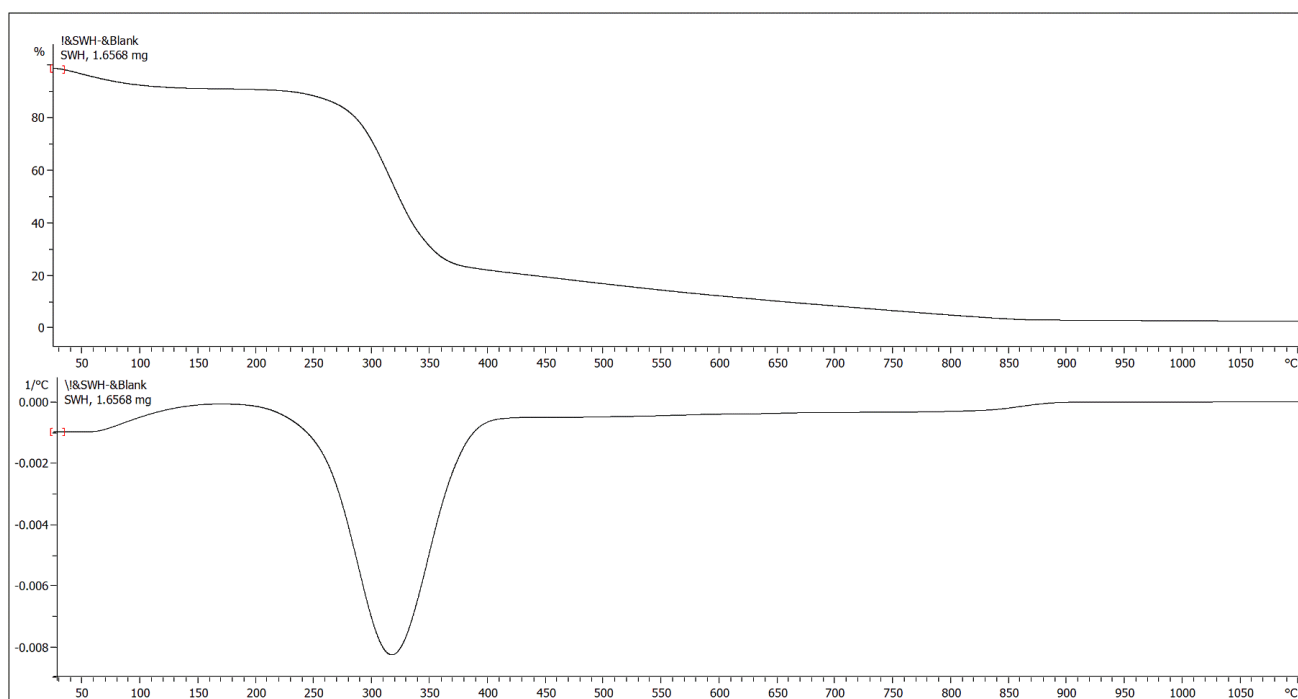
Figure S1 TGA and DSC curves of raw sago hampas.
