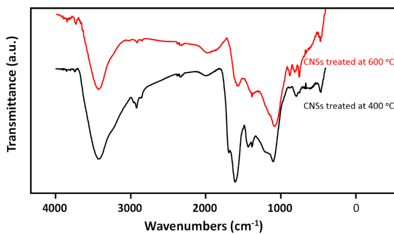
Fig. S4 FT-IR spectra of CNSs at 400 °C and 600 °C.
