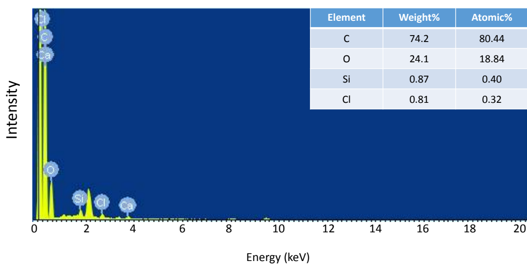
Fig. S2 EDX spectrum for CNSs pyrolyzed at 400 °C.
