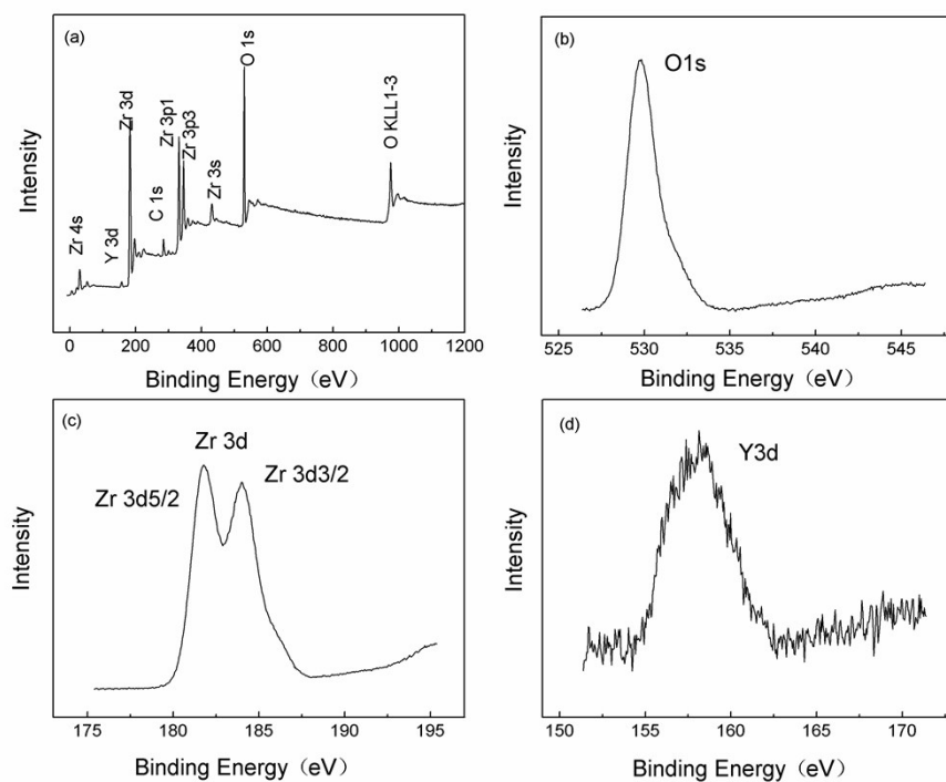
Fig. S3 XPS of 8YSZ
