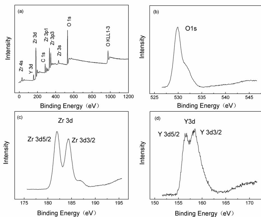
Fig. S5 XPS of 50YSZ
