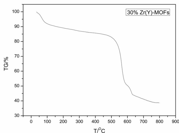
Fig. S1 TG curve of MOFs
