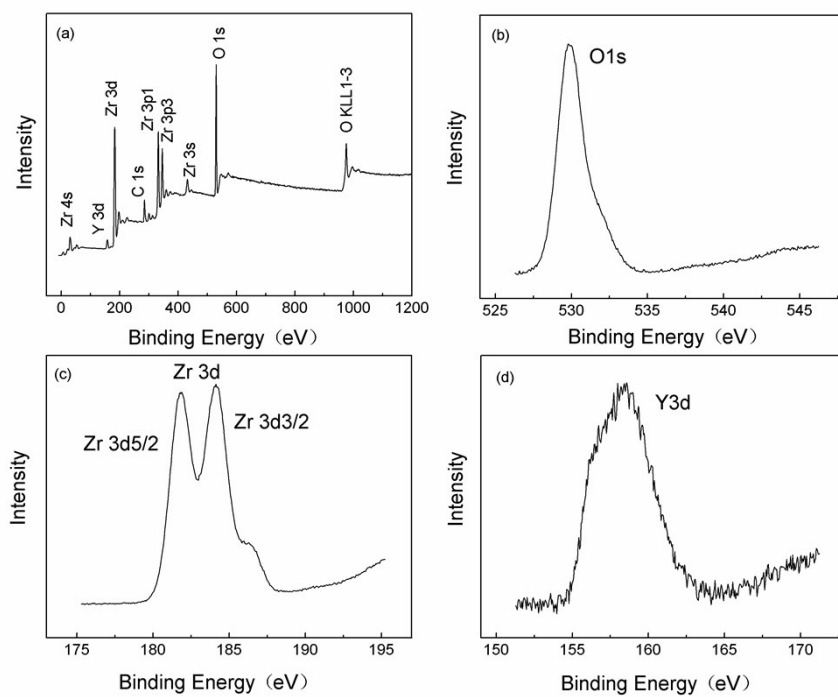
Fig. S4 XPS of 30YSZ
