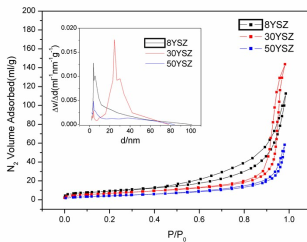
Fig. S6 Nitrogen adsorption-desorption isotherms and pore size distribution curves (inset) of YSZ
