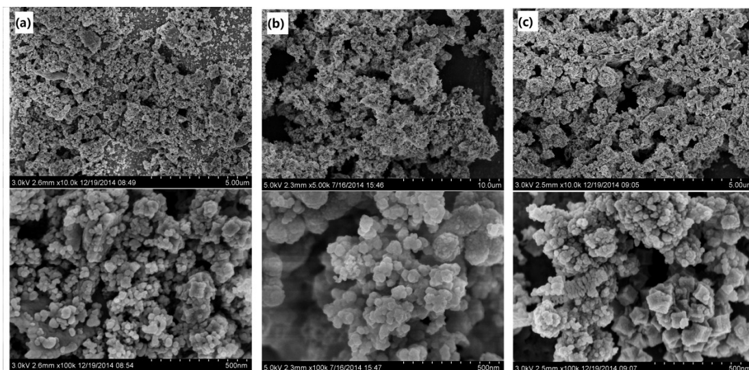
Fig. S2 SEM images of samples: (a)8YSZ; (b)30YSZ; (c)50YSZ
