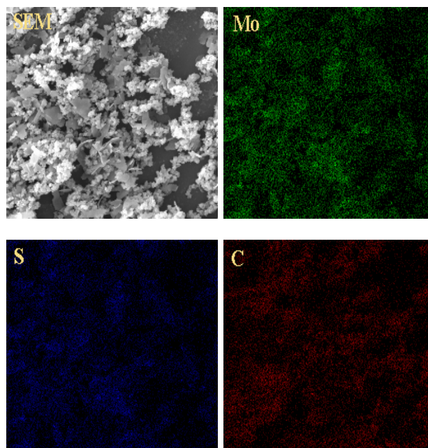
Fig. S1. SEM image of MoS 2 -C and the EDX mapping images of Mo, S, and C elements.
