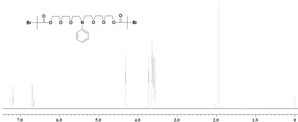
Fig. S1 1 H NMR spectrum of ATRP initiator in CDCl 3
