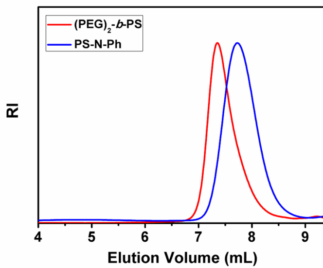
Fig. S3 GPC traces of PS-N-Ph (PDI=1.29, M_n =8800) and (\text{PEG})_2 - b -PS (PDI=1.28, M_n =13500).
