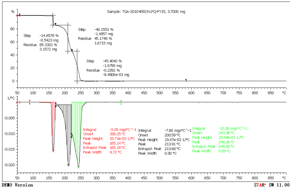
The TGA and DSC curve of 4
