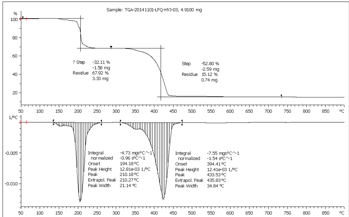
The TGA and DSC curve of 5
