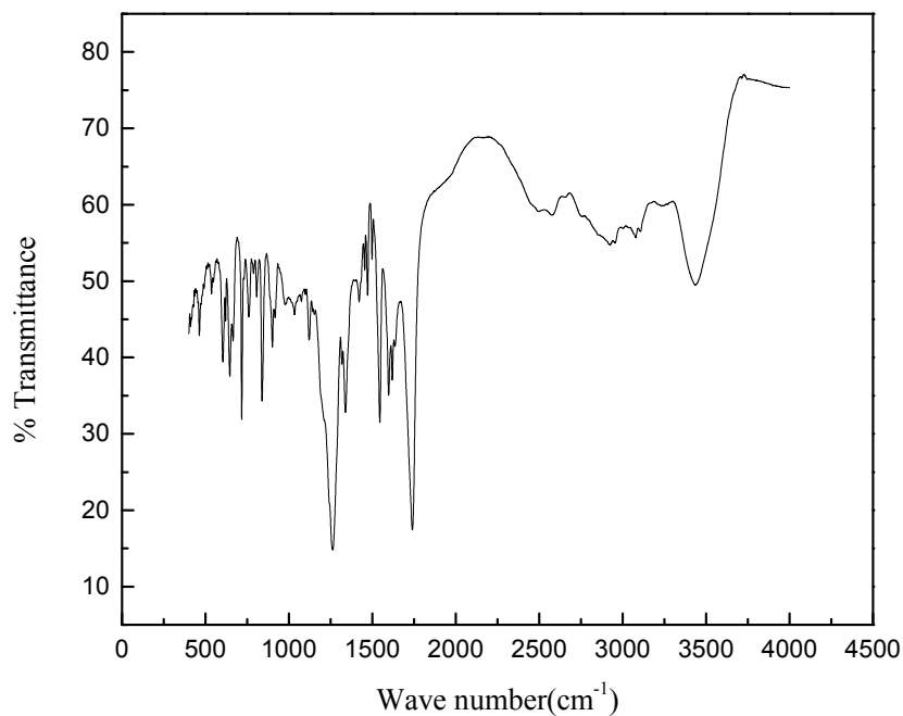
The IR curve of 1
