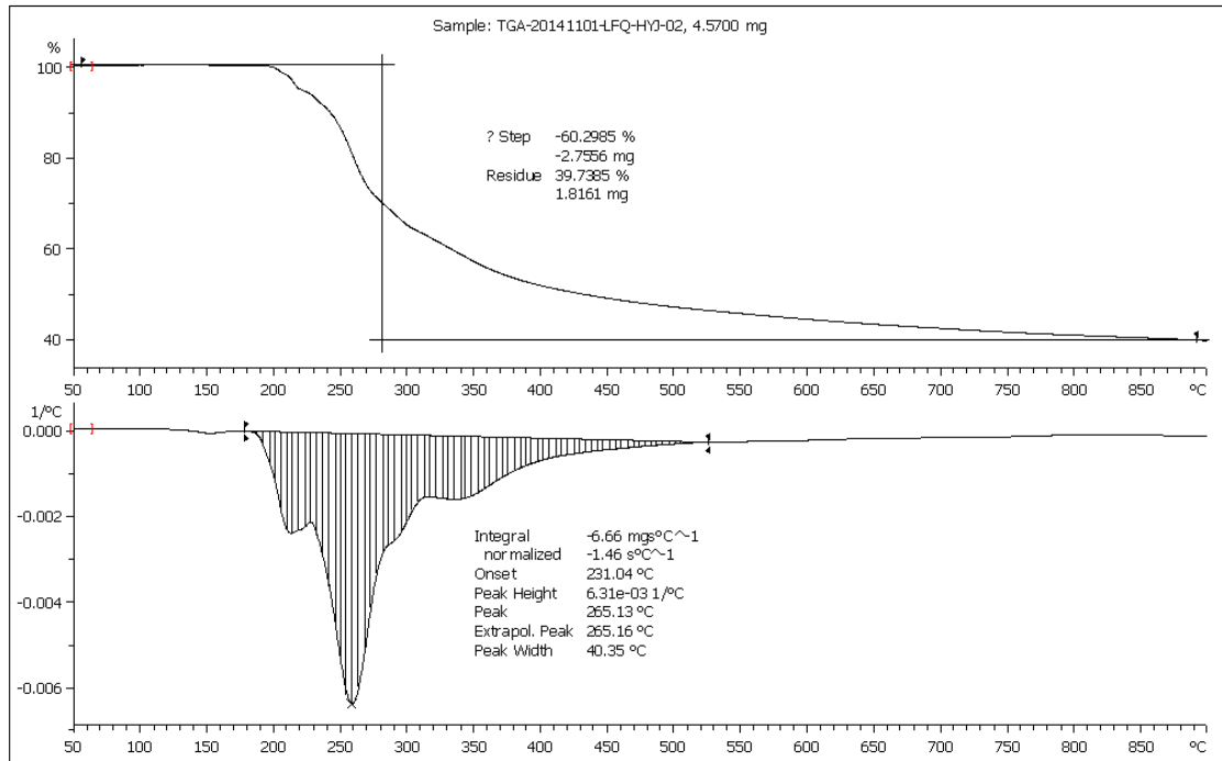
The TGA and DSC curve of 3
