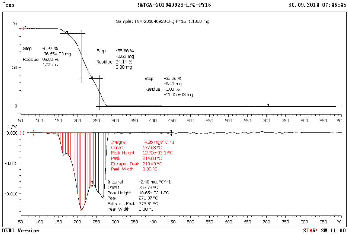
The TGA and DSC curve of 1
