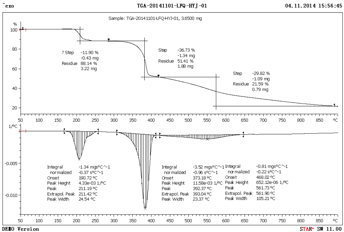
The TGA and DSC curve of 2
