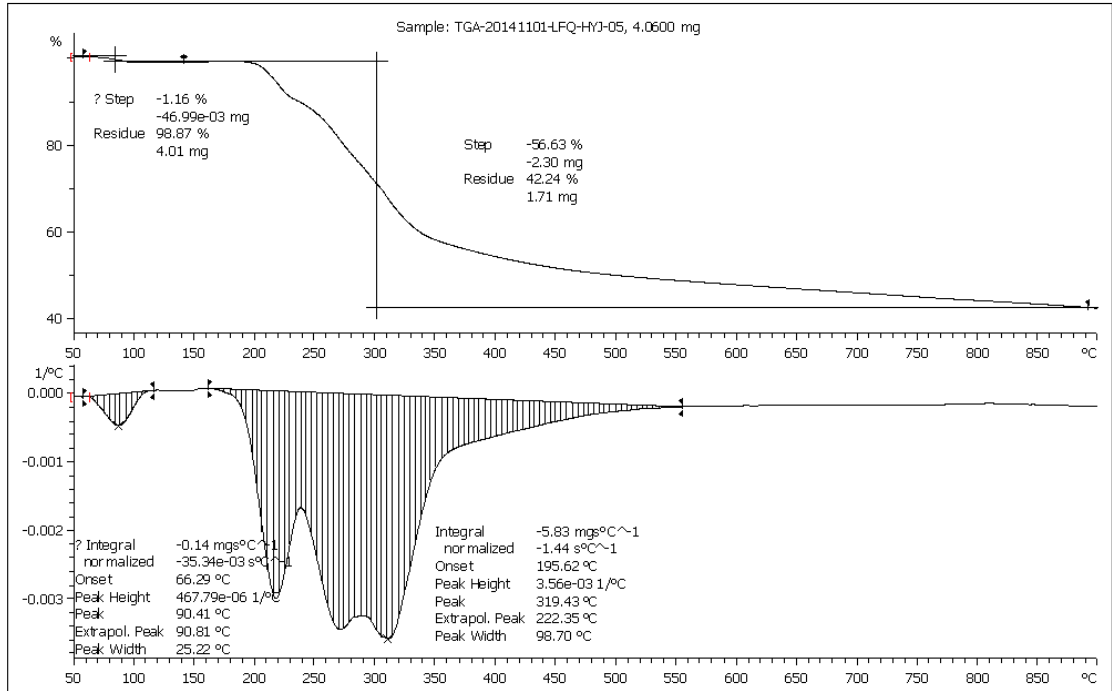
The TGA and DSC curve of 7
