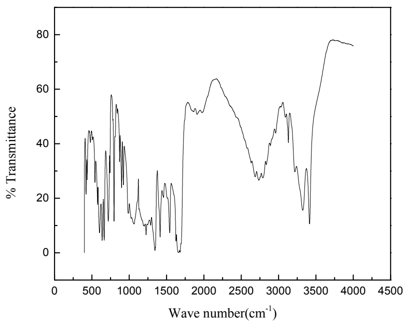
The IR curve of 4
