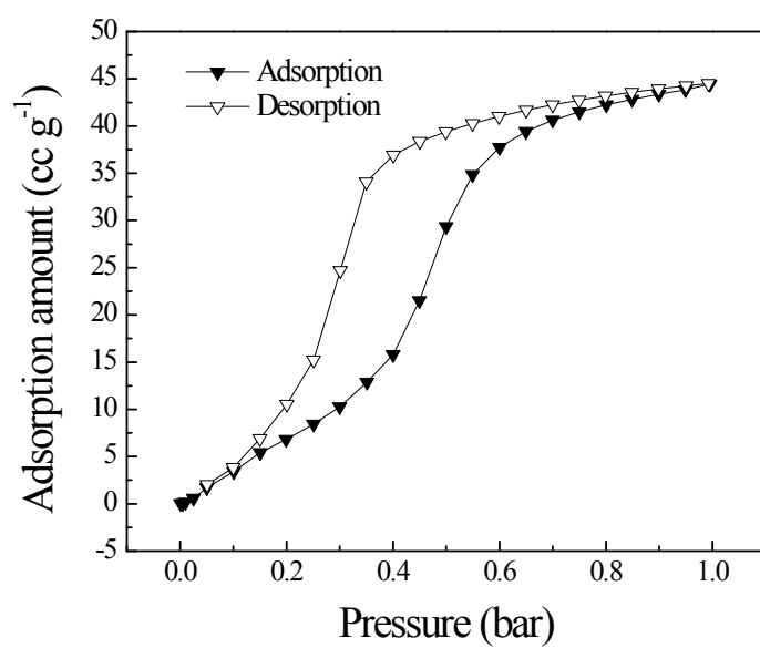
Fig. S2 CO 2 adsorption isotherm of the ZIF-7 powder at 298 K.
