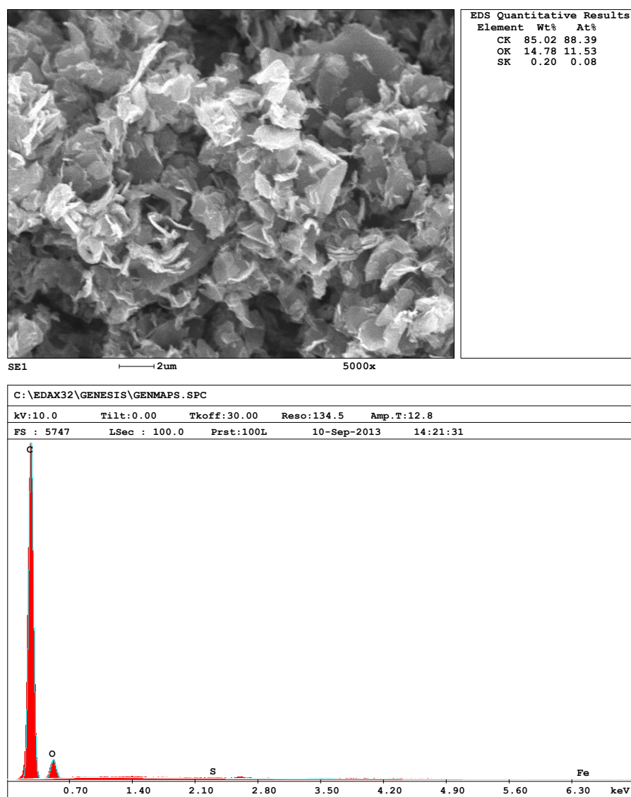
Figure S1. EDX spectrum of Fe-rGO.
