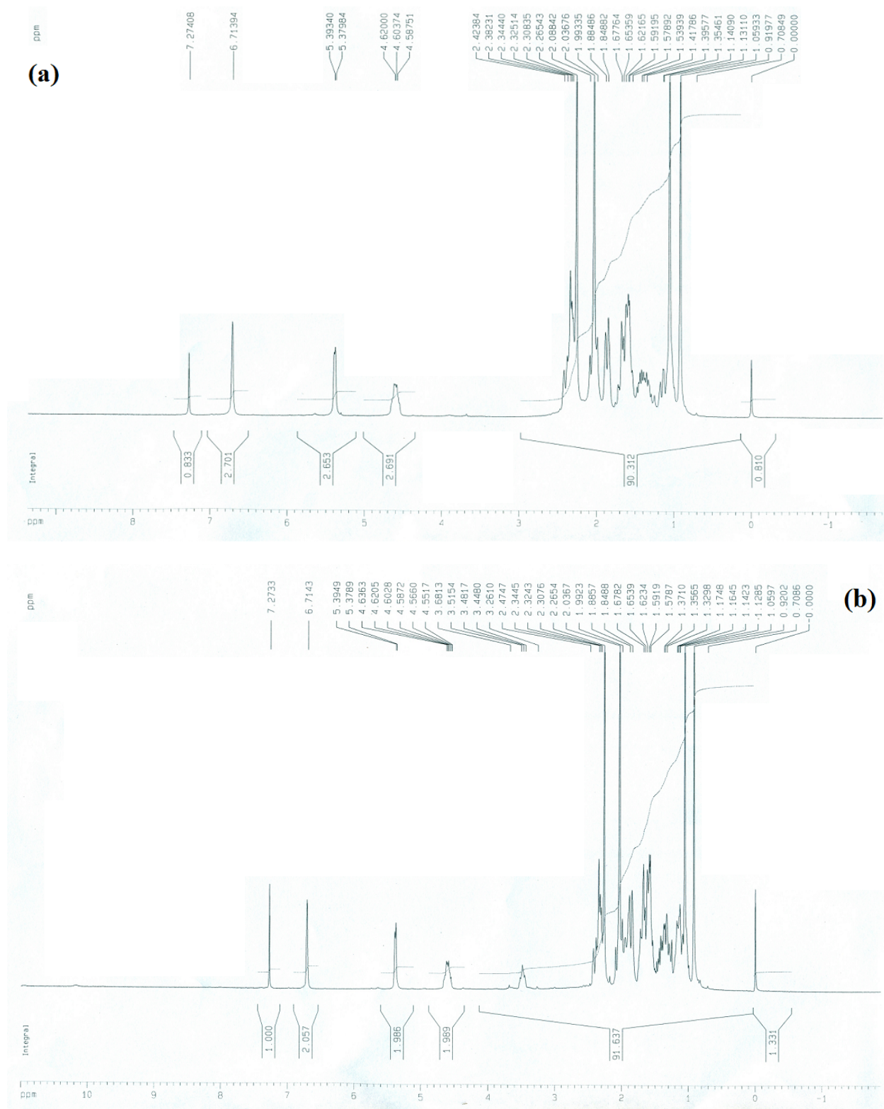
Figure 1 : ^1\text{H} NMR spectra (a) 16-DPA (b) Chitosan-16DPA.
