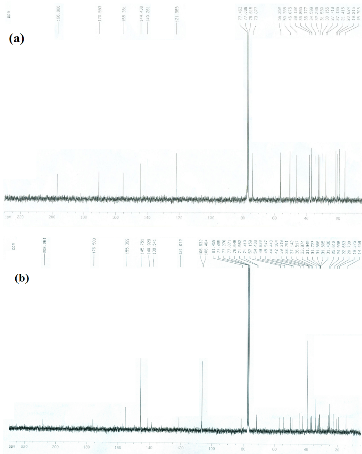
Figure 2 : ^{13}\text{C} NMR spectra (a) 16-DPA (b) Chitosan-16DPA.
