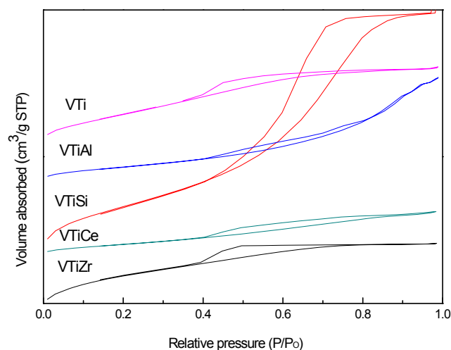
Fig. S1. N 2 adsorption and desorption isotherms of the VTi, VTiAl, VTiSi, VTiCe and VTiZr samples.
