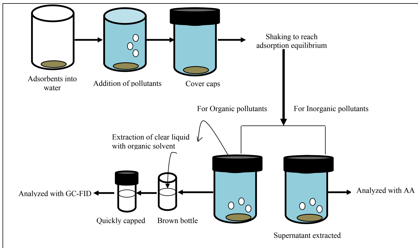
Fig. S2: Schematic representation of adsorption experiments
