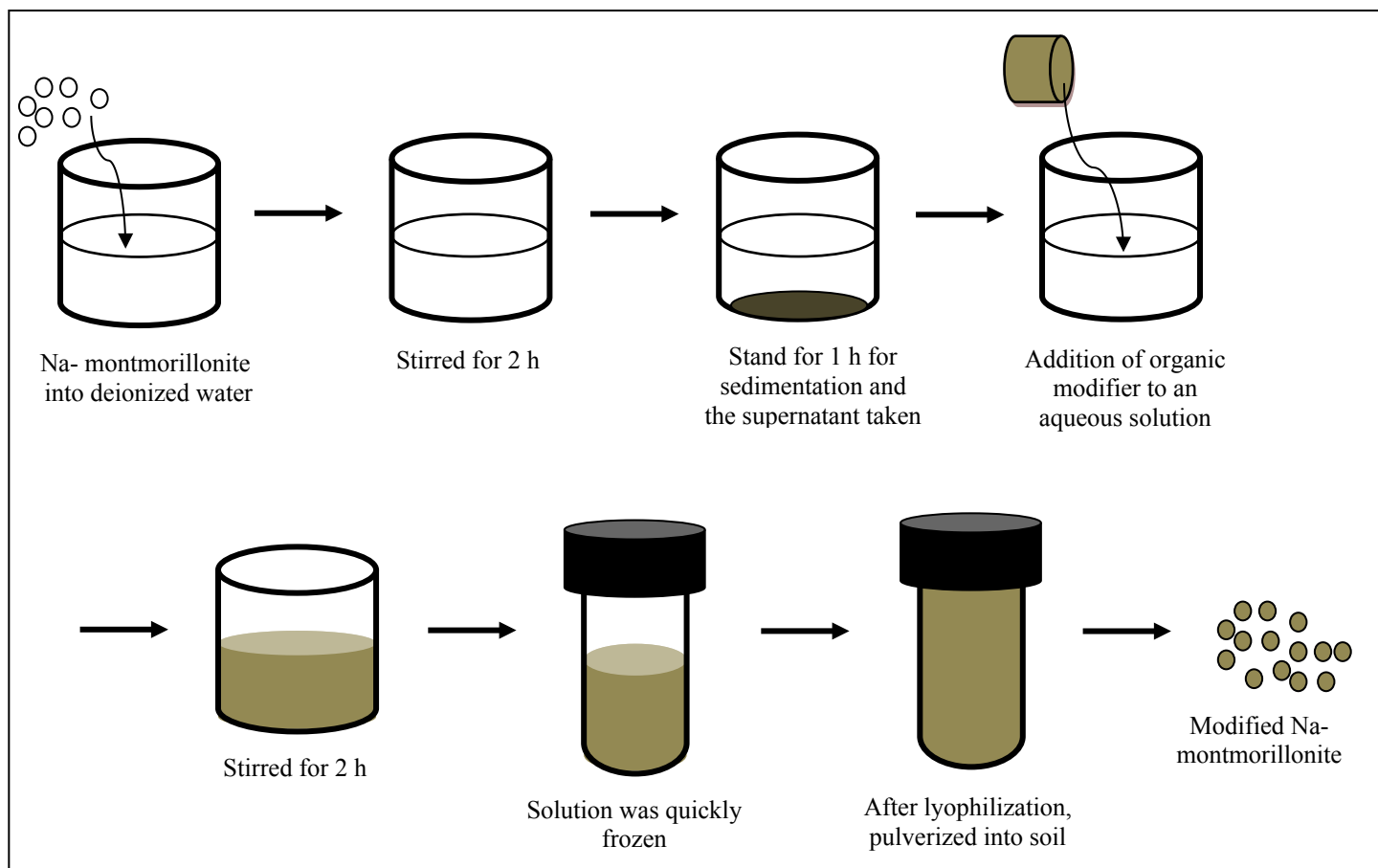
Fig. S1: Modification of Na-montmorillonite by different modifiers
