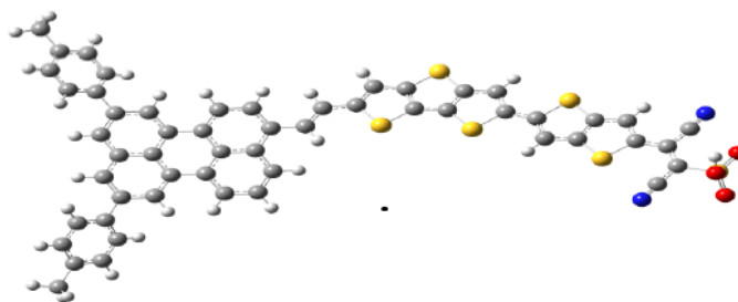
Figure S1. The optimized geometric structures of d01-d12 and BUCT7- BUCT12
