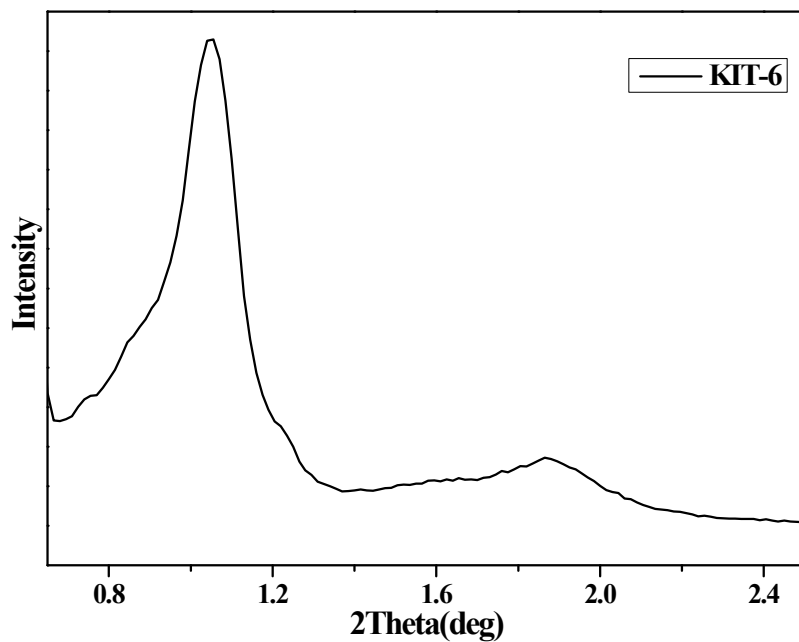
Figure 1S. Low-angle XRD pattern of KIT-6
