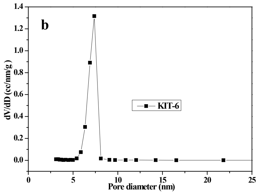
Figure 2S. N 2 adsorption-desorption isotherms (a) and pore diameter distribution (b) of KIT-6.
