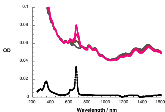
Figure S2 Absorption spectra of 1 (black), SWNT suspended in THF (grey) and titration of these SWNT with 1 (brown to purple).
