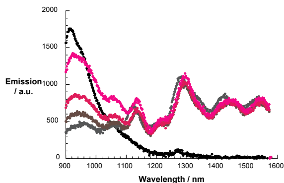
Figure S1 NIR fluorescence spectra of 1 (black), SWNT suspended in THF (grey) and titration of these SWNT with 1 (brown to purple).
