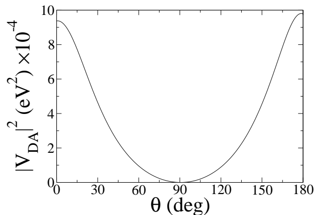
Fig. ESI 4 The squared excitonic coupling |V_{DA}|^2 between two chromophores as a function of their relative orientation and distance of 8.5\text{\AA} , which corresponds to the average distance between first nearest neighbors within the smectic layers at 300 K.
