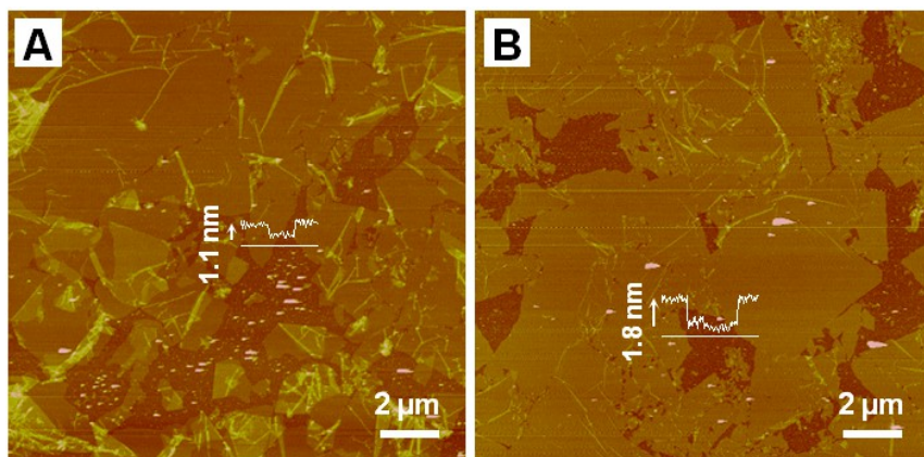
Fig. S1 AFM images of rGO sheets on Si substrate before (A) and after (B) adsorption of R6G.
