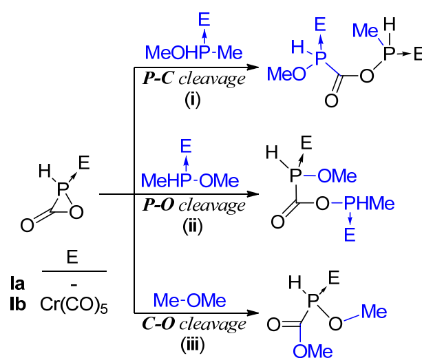
Scheme SI 1. Homodesmotic reactions used (as average) to evaluate RSE for compounds la , b .
