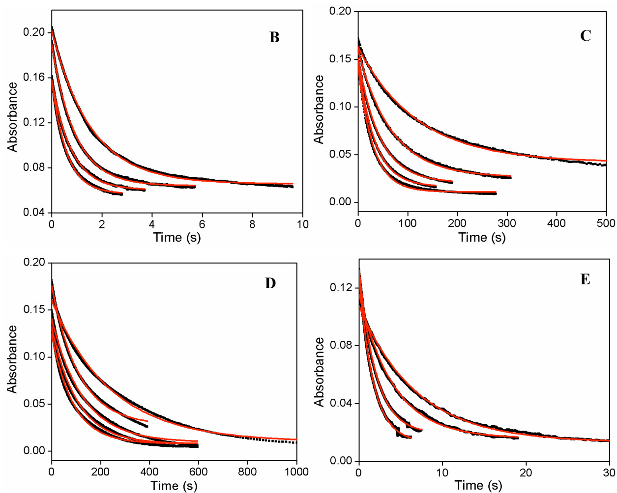
Figure S9c. Kinetic traces (black points) in the course of their reactions with DHA for \text{Fe}^{\text{IV}}=\text{O} complexes 2 (B), 3 (C), 4 (D) and 5 (E) in \text{CH}_3\text{CN} at 25^\circ\text{C} .
