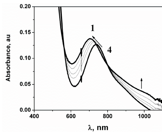
Figure S8. Spectral changes associated with the oxo-transfer reaction between 4 and 1a in CH 3 CN at 25 °C yielding 1 quantitatively.
