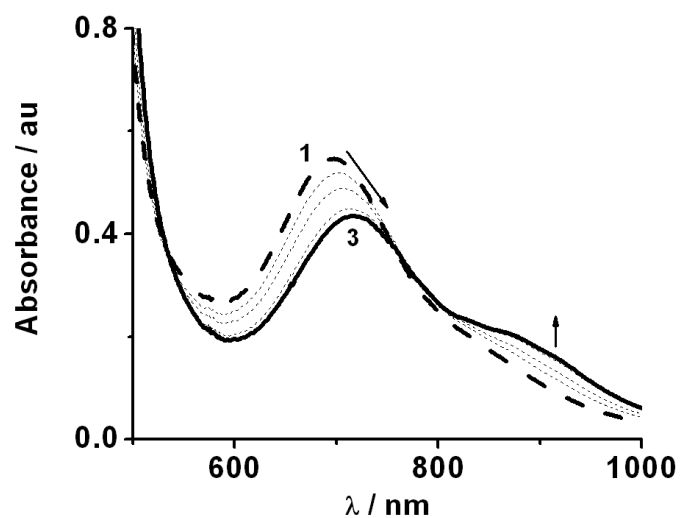
Figure S6. Spectral changes showing the oxo-transfer reaction between 1 and 3a in CH 3 CN at 25 °C to yield 3 quantitatively
