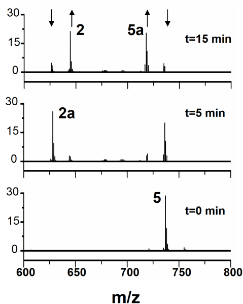
Figure S7. ESI-MS spectral changes associated with the oxo-transfer reaction between 5 and 2a in CH 3 CN at 25 °C to yield the respective complexes 5a and 2 .
