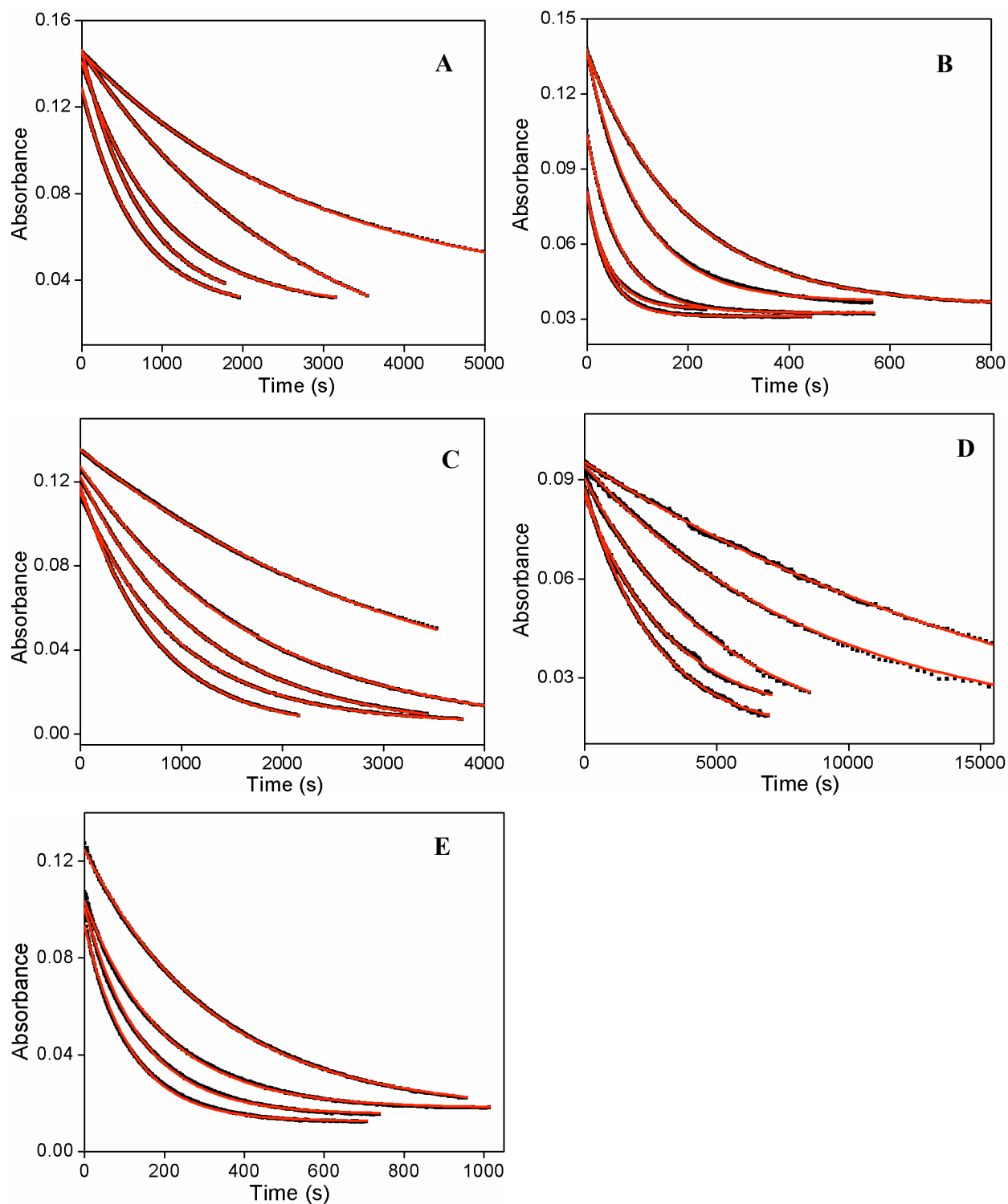
Figure S9b. Kinetic traces (black points) in the course of their reactions with CHD for \text{Fe}^{\text{IV}}=\text{O} complexes 1 (A), 2 (B), 3 (C), 4 (D) and 5 (E) in \text{CH}_3\text{CN} at -40^\circ\text{C} .
