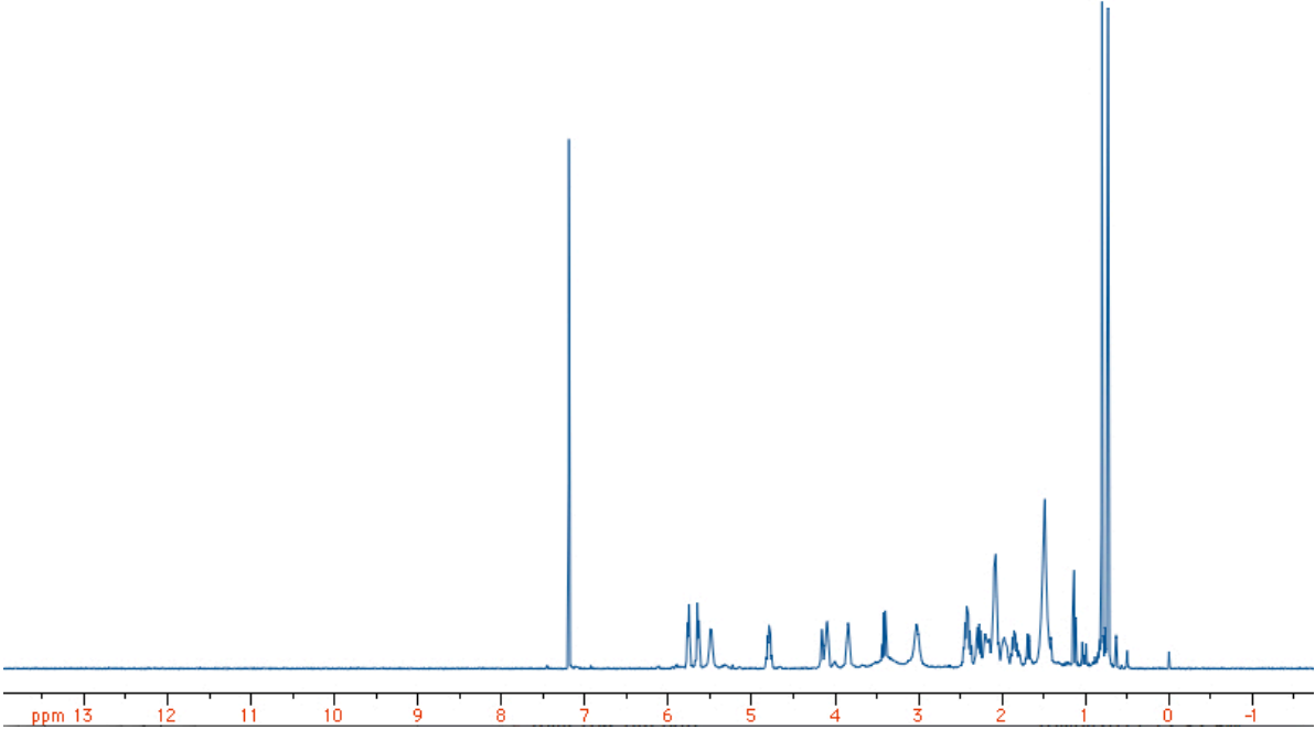
1 H NMR Rh(cod)Cl•CKphos
