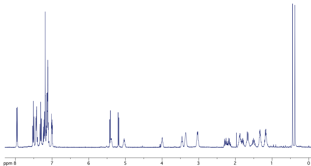
^1\text{H-NMR} \text{Rh(cod)Cl}\cdot\text{T1}
