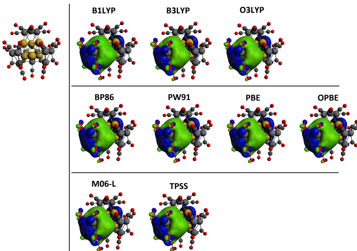
Figure S1. Representative Localized Molecular Orbital for superatomic SP3 hybrids at several levels of theory involving Hybrid, GGA and Meta-GGA functionals, employing STO-TZ2P and ZORA scalar relativistic hamiltonian. Isosurfaces at \pm 0.01 a.u..
