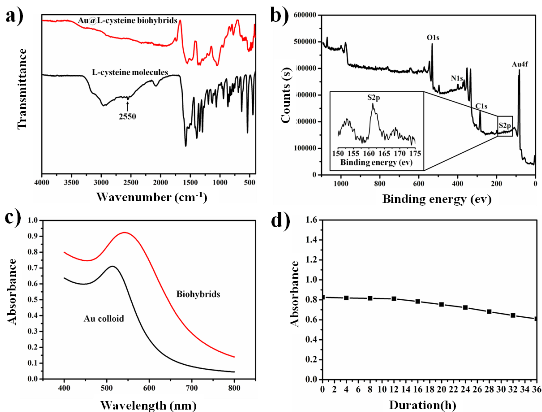
Supplementary Figure S2 a) FTIR spectra of biohybrids (top) and L-cysteine (bottom; b) XPS spectrum of biohybrids and the narrow scan of S 2p (inset) with a binding energy of 162 eV; c) UV-vis spectra of Au colloid (bottom) and biohybrids (top) and d) the stability of biohybrids.
