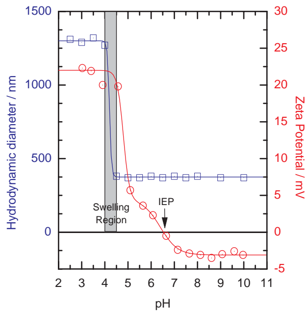
Fig. S1. Bulk hydrodynamic diameter and zeta potential for the PEGMA stabilised P2VP microgel. The swelling region is between pH 4.0 and 4.5 and isoelectric point at pH 6.5. Solid lines are a guide to the eye only.
