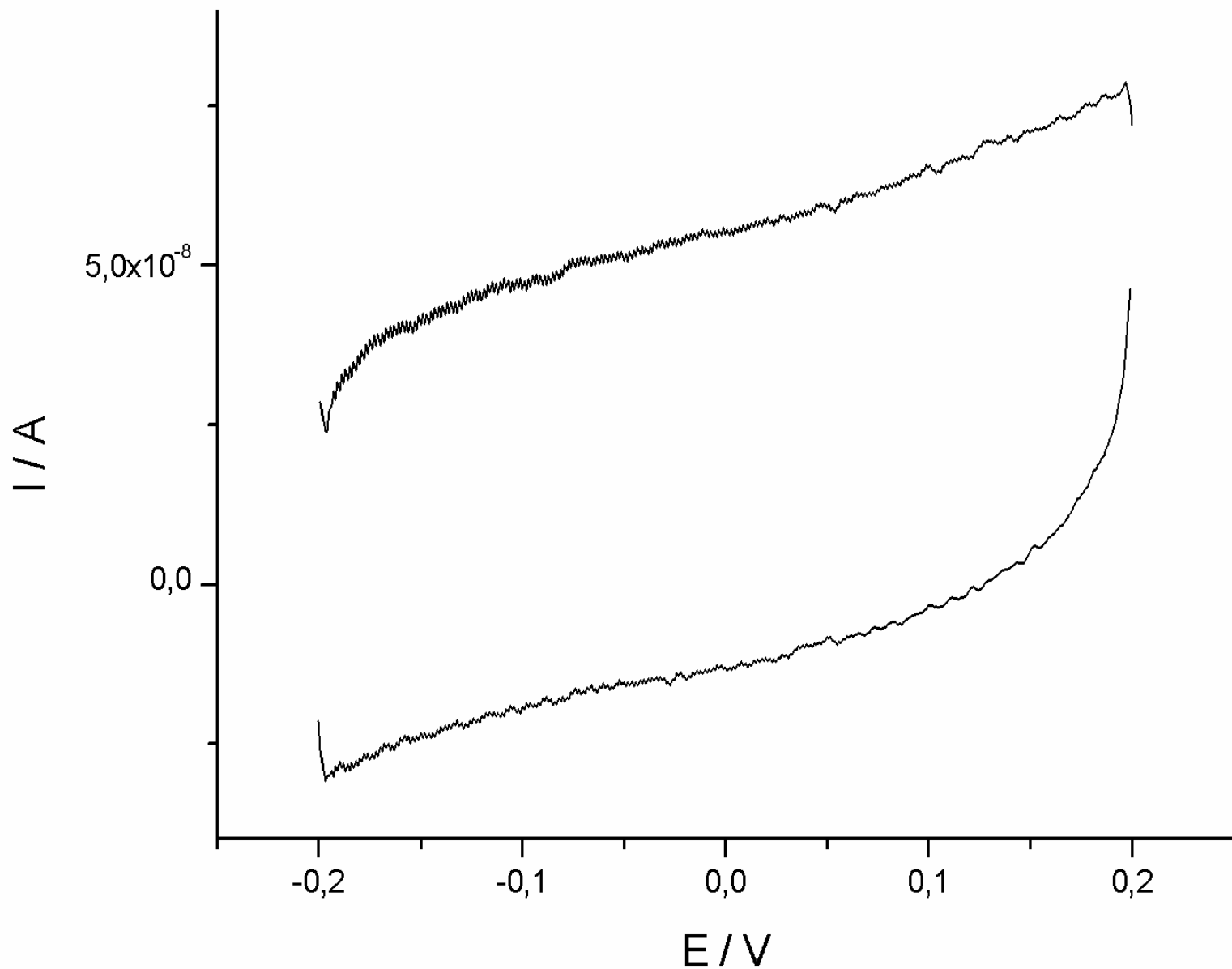
Fig. S1 CV of 0.2 \text{ mg mL}^{-1} PASA in 5 \text{ mM Tris} , 2 \text{ mM KCl} pH 8.5 on Au-Mu/MuA. at 0.1 \text{ V s}^{-1} .
