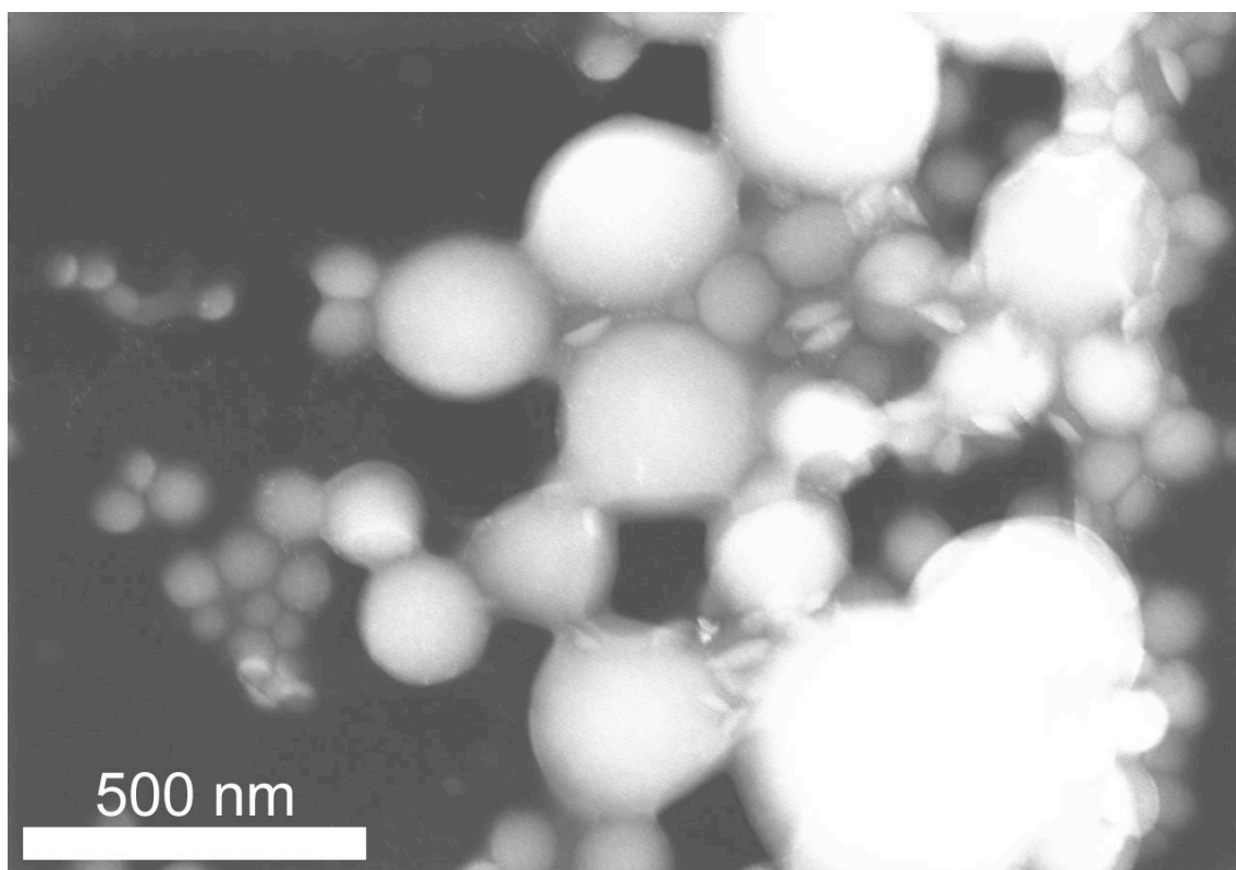
S-1. STEM image (dark field TEM mode) of the nanoparticles containing PSt and PI prepared by reprecipitation method.
