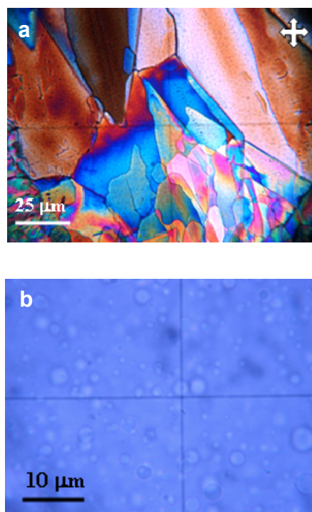
Fig.S2. a) Gelly phase under crossed polarizers of 1:1 BDSA-6ACA with characteristic interference hues b) Spherical vesicles from 1:1 BDSA-4ABA .
