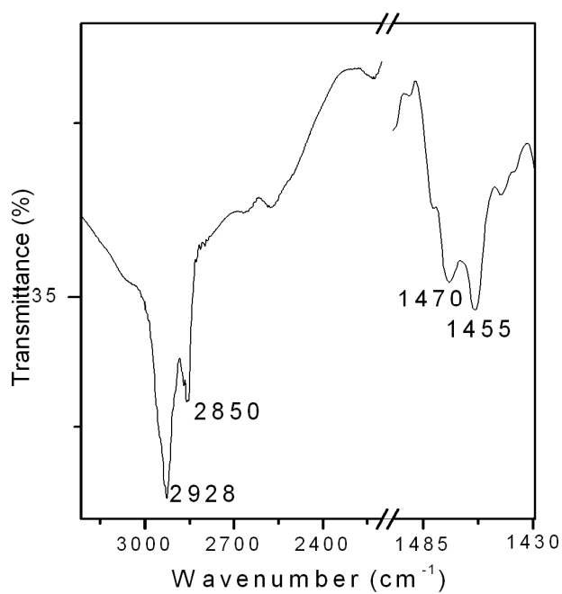
Fig.S3. FT-IR of 1:2 BDSA-6ACA gel phase.
