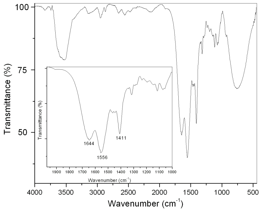
Fig.S4. FT-IR of 6-amino caproic acid.
