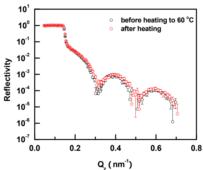
Figure S2. Neutron reflectometry curves from a sample with structure Si/PEI/(PSS/PAH) 6 before and after temperature treatment at 60 °C for 1 hour. No difference in the reflectivity at room temperature was observed before and after the temperature treatment. The result proves that no changes occurred in the sample after the treatment.
