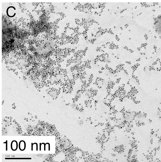
Figure 1: Supplementary TEM images of gold nanoparticles : A) R_w=1 , h = 10 ; B) R_w=2 , h = 10 ; C) R_w=2 , h = 5 .
