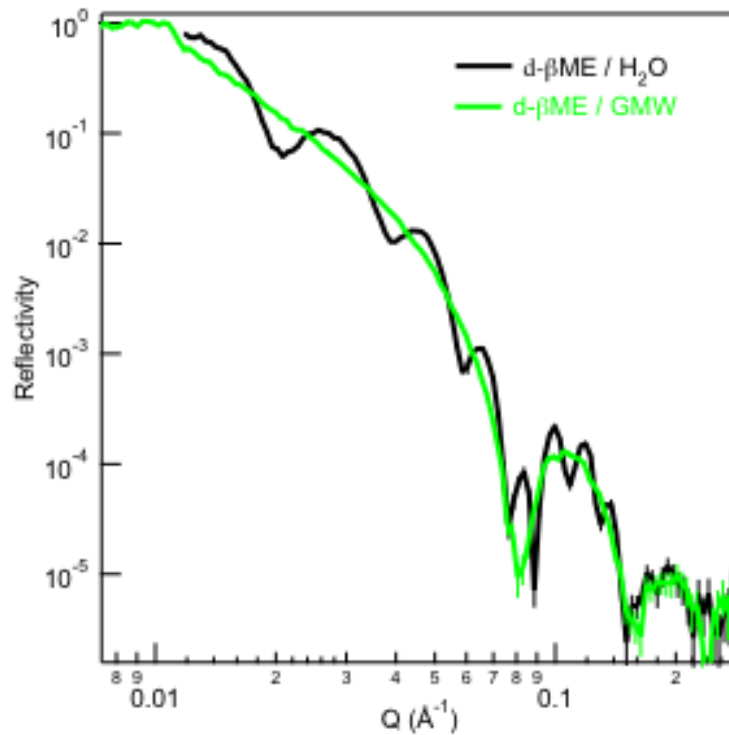
Figure S1. Reflectivity datasets, “up” spin state only for different \beta ME contrast conditions. Data presented as lines between points to enable ready tracing of the fringes. The minima of the broad fringe ( \sim 0.08 and 0.15 \text{ \AA} ) is due to the thickness of the magnetic reference layer. The critical edge it is at \sim 0.1 \text{ \AA}^{-1} for gold matched water (GMW), green, buffer and is absent for \text{H}_2\text{O} buffer, black, where the change in nSLD from the silicon to the buffer is negative. The absence of small fringes in the GMW dataset is because the buffer contrast is matched to the gold, which approximates the nSLD of the d- \beta ME. When the buffer is replaced with \text{H}_2\text{O} the small fringes are evident as the gold and d- \beta ME layers are now visible.
