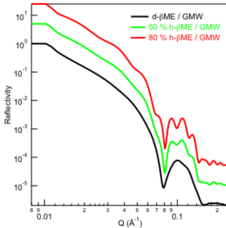
Figure S2. Simulated reflectivity datasets based upon the fits for data shown in Fig. S1 with simulations offset for clarity. Black – simulated version of d- \beta ME with GMW subphase, note the asymmetry in shape of the fringe (maximum \sim 0.1 ) is because the d- \beta ME does not exactly match the gold nSLD. Green simulation is for the same gold and magnetic layer structure and GMW buffer but with the surface covered with 50 % h- \beta ME. Red simulation is with increased h- \beta ME surface coverage. The simulations clearly illustrate the sensitivity of the data to the surface adsorption of very thin layers of hydrogenous material.
