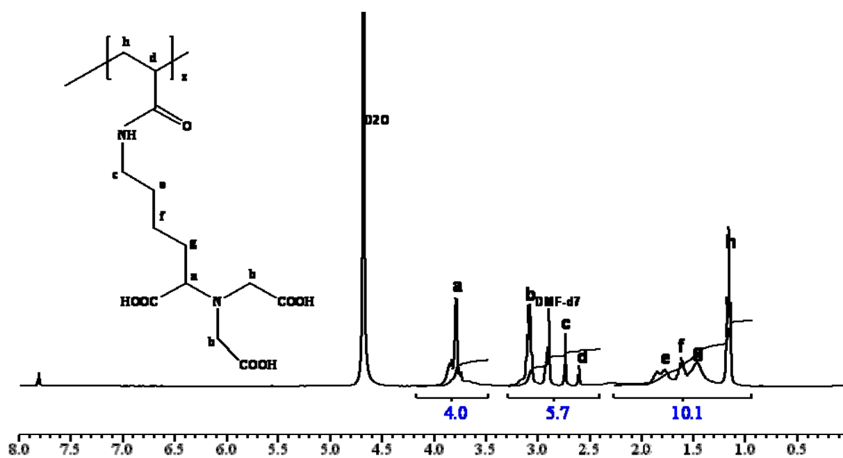
Supplementary Figure 1. ^1\text{H} NMR spectrum of the polymeric ligand
