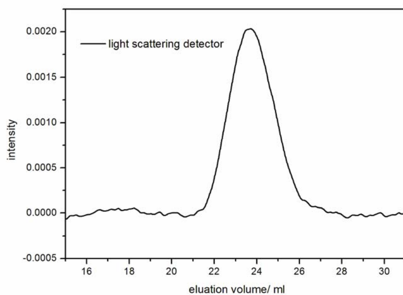
Supplementary Figure 3. GPC data of the polymeric ligand.
