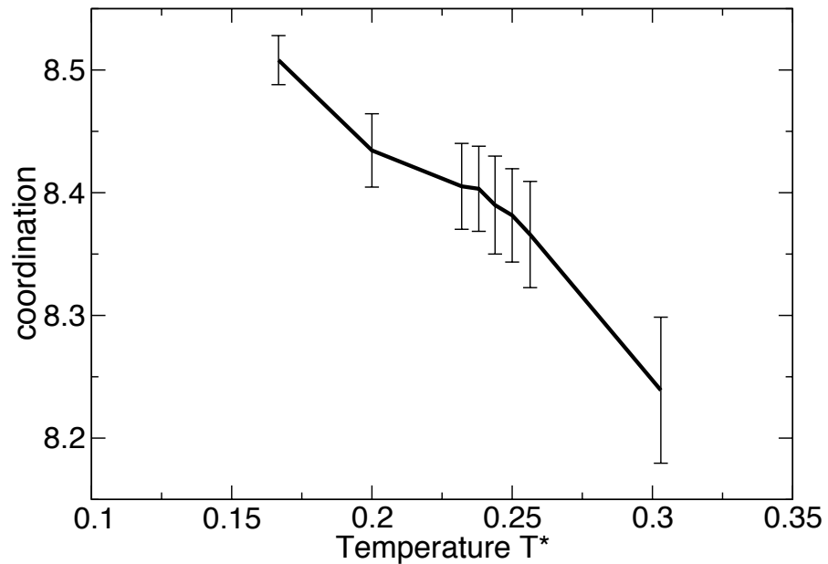
Voronoi S Tessellation
