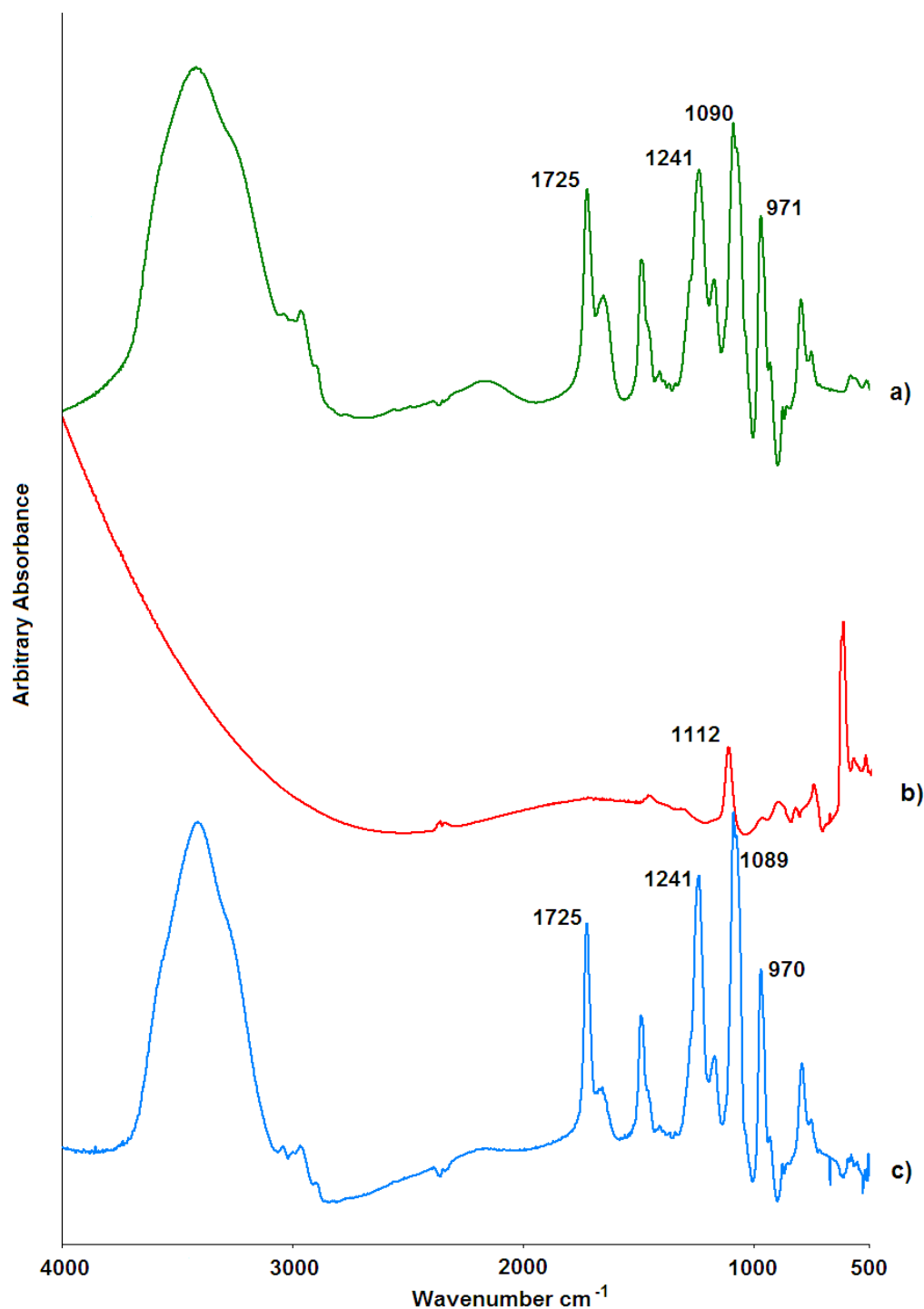
Figure S1. FT-IR spectra of: (a) PMPC homopolymer (KBr disc); (b) bare planar silicon wafer; (c) PMPC-coated silicon wafer. All spectra were recorded in transmission mode. Spectra have been vertically offset for clarity.
