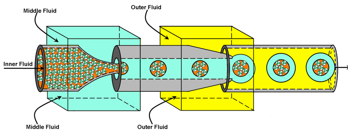
Fig. S1. Schematic illustration of the microfluidic device.
