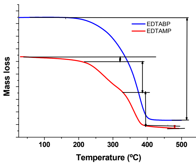
Fig. 2S TGA of EDTA-MP and EDTA-BP at a scan rate of 10 °C/min.
