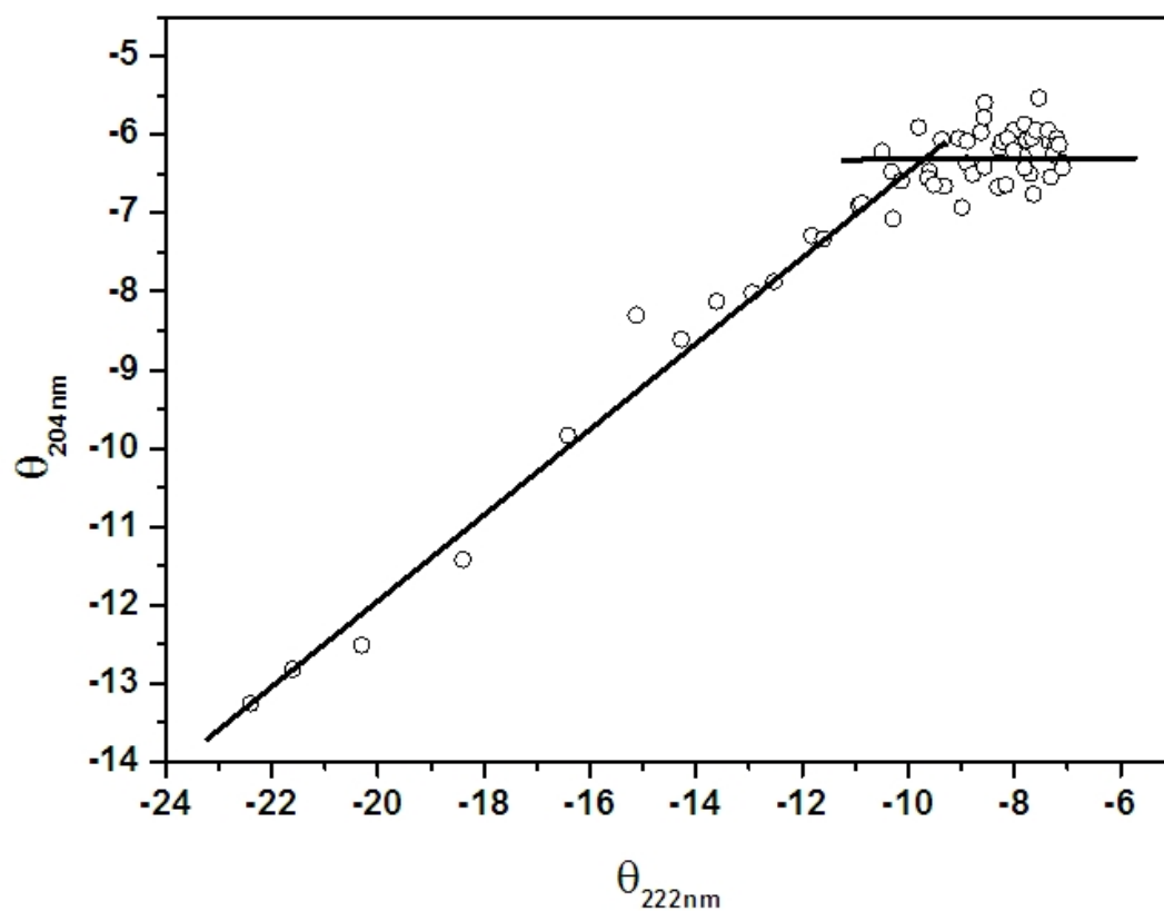
Phase diagram showing a two-state conformational transition during \alpha -PLL unfolding in strong shear regions.
