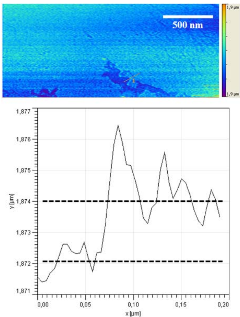
Figure X2. Detail of membrane thickness of the ABA block copolymer layer deposited onto solid glass support.
