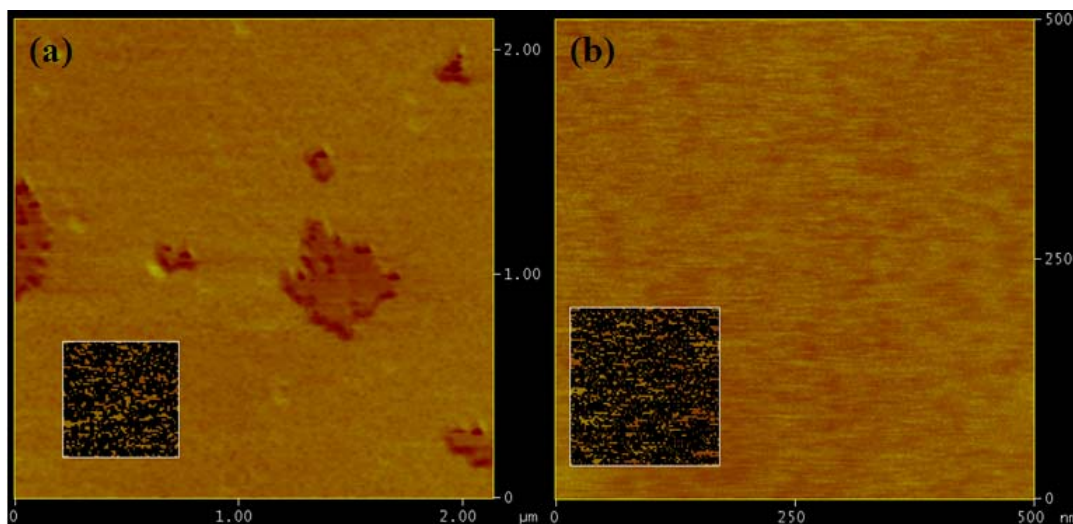
Figure X3. Different regions of the (a) block copolymer membrane and (b) clean mica used for the determination of their mean roughness. In (a) 0.108 nm, polymer membrane, and (b) 0.571 nm, mica.
